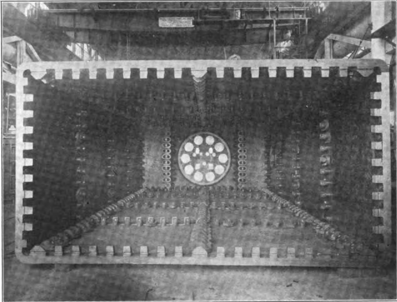
FIG. 7.—INTERIOR OF MANGANESE STEEL VAULT CONSTRUCTED FOR THE FEDERAL SAFE DEPOSIT CO., NEW YORK. 16' 8" Wide Without Supporting Columns.
