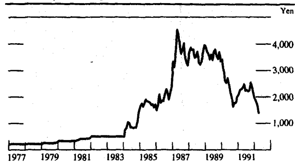
3. Price of a share of Sumitomo Bank, January 1977–April 1992 1
